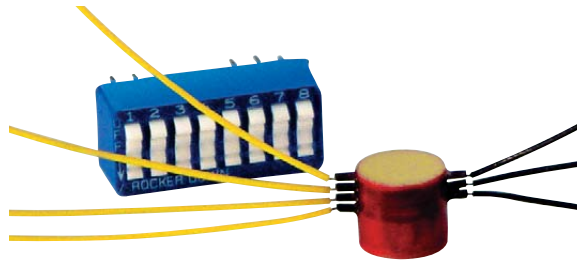
Custom PICA™-Stack actuator, each layer wired individually.
